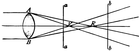
FIG. 56.—Chromatic aberration.
